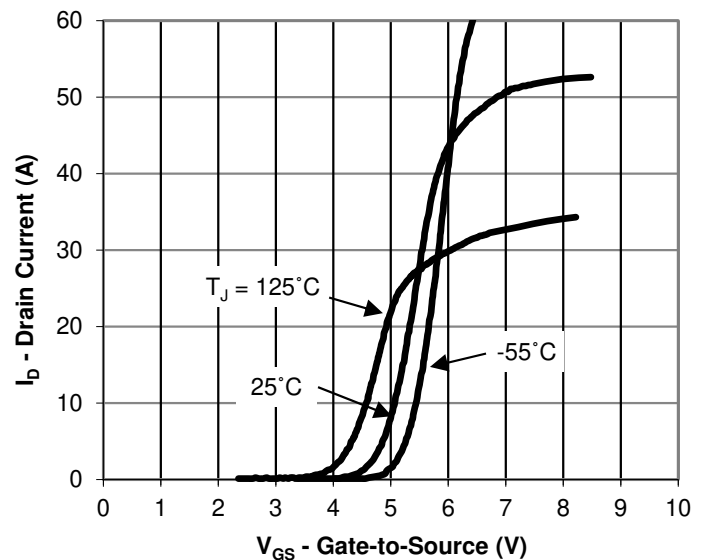
Transfer Characteristics
