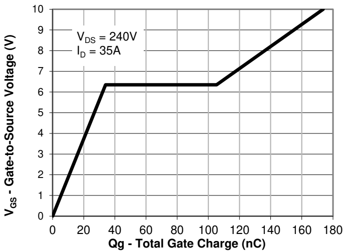
Gate Charge
