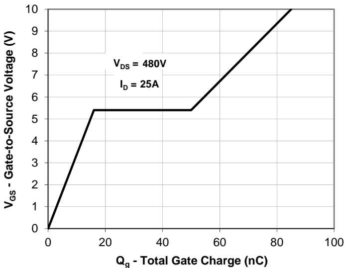
Gate Charge
