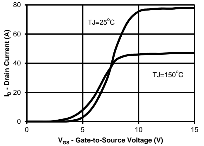
Transfer Characteristics
