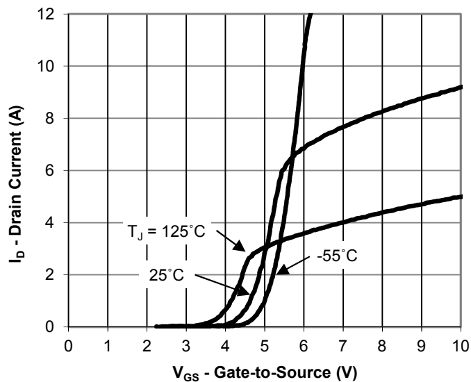
Transfer Characteristics
